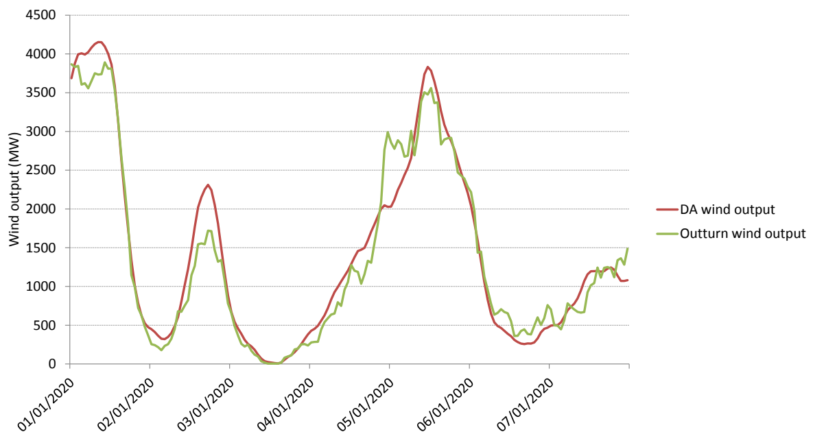
Figure 6 – Outturn and expected Day-Ahead wind output for the whole island of Ireland for a sample week in January 2020 (weather year 2006)
