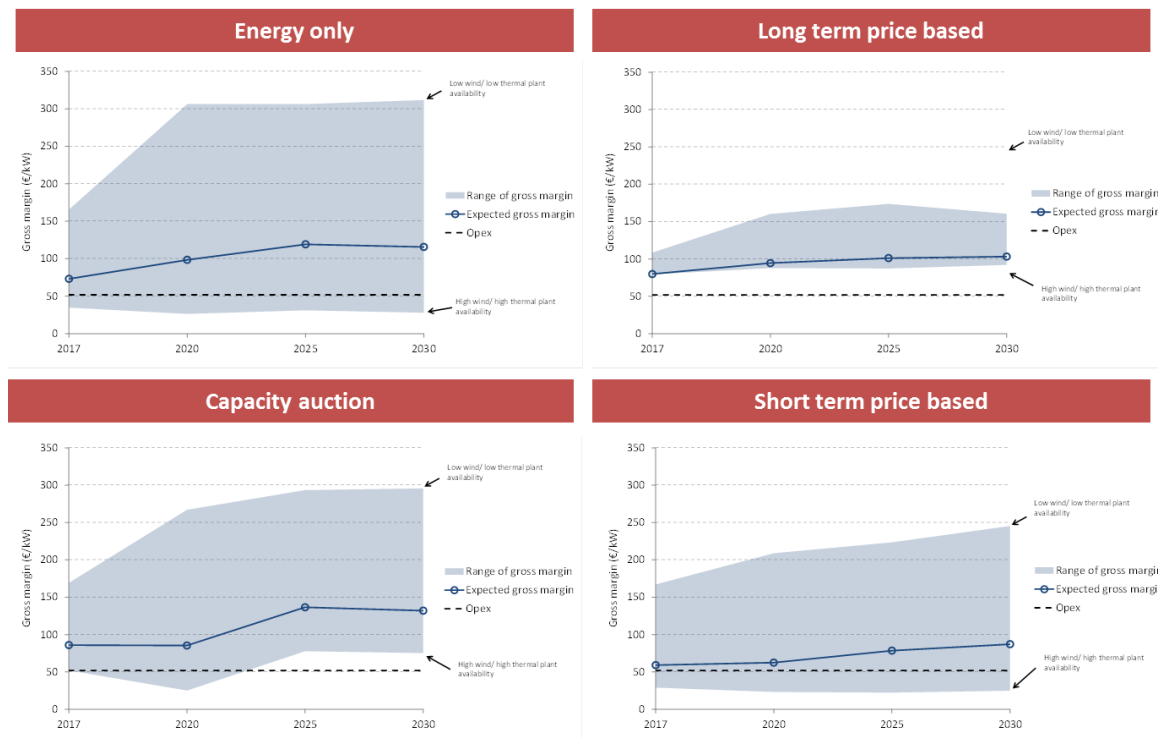
Figure 18 –Gross margin 42 for a 51% efficient (HHV) CCGT under the energy-only market and different types of CRMs (Base Case A)
