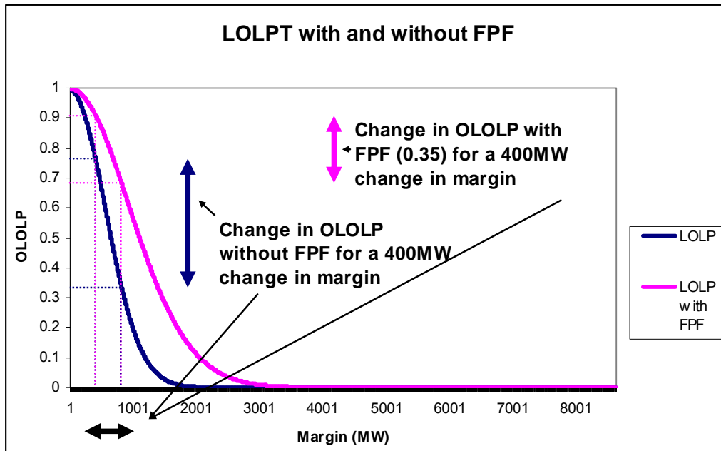
Fig. 3.1. – LOLP Curve with and without FPF
