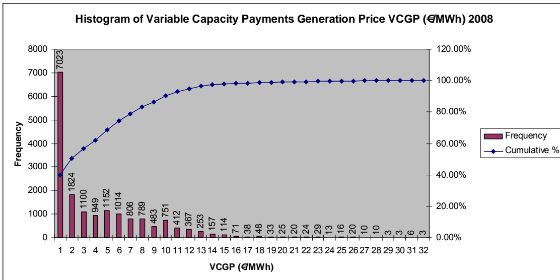
Fig. 4.3a – Histogram of Variable Capacity Payments Generation Price
